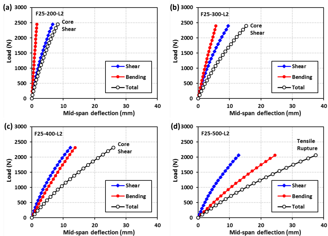
Figure 14. Effect of span length on the behavior of foam-filled paper honeycomb
