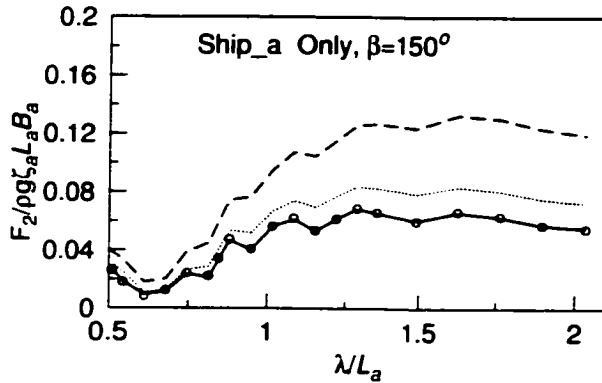
Sway force on ship_a at a separation Gy=2000.0m, dx=0.0m, U=0.0m/s
