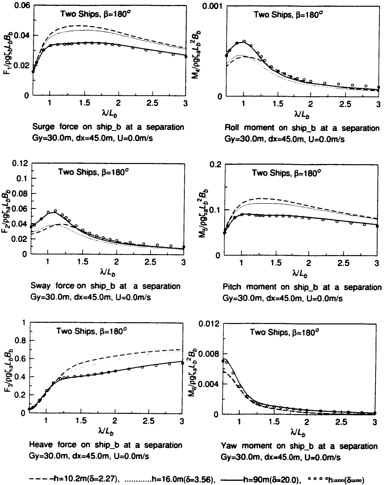
Figure 5.34: Non-dimensional wave exciting force amplitudes on ship_b in Case 2
