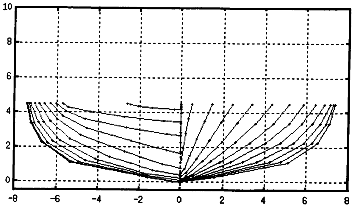
Figure 5.16: Body plan of the ship_b hull (frigate)
