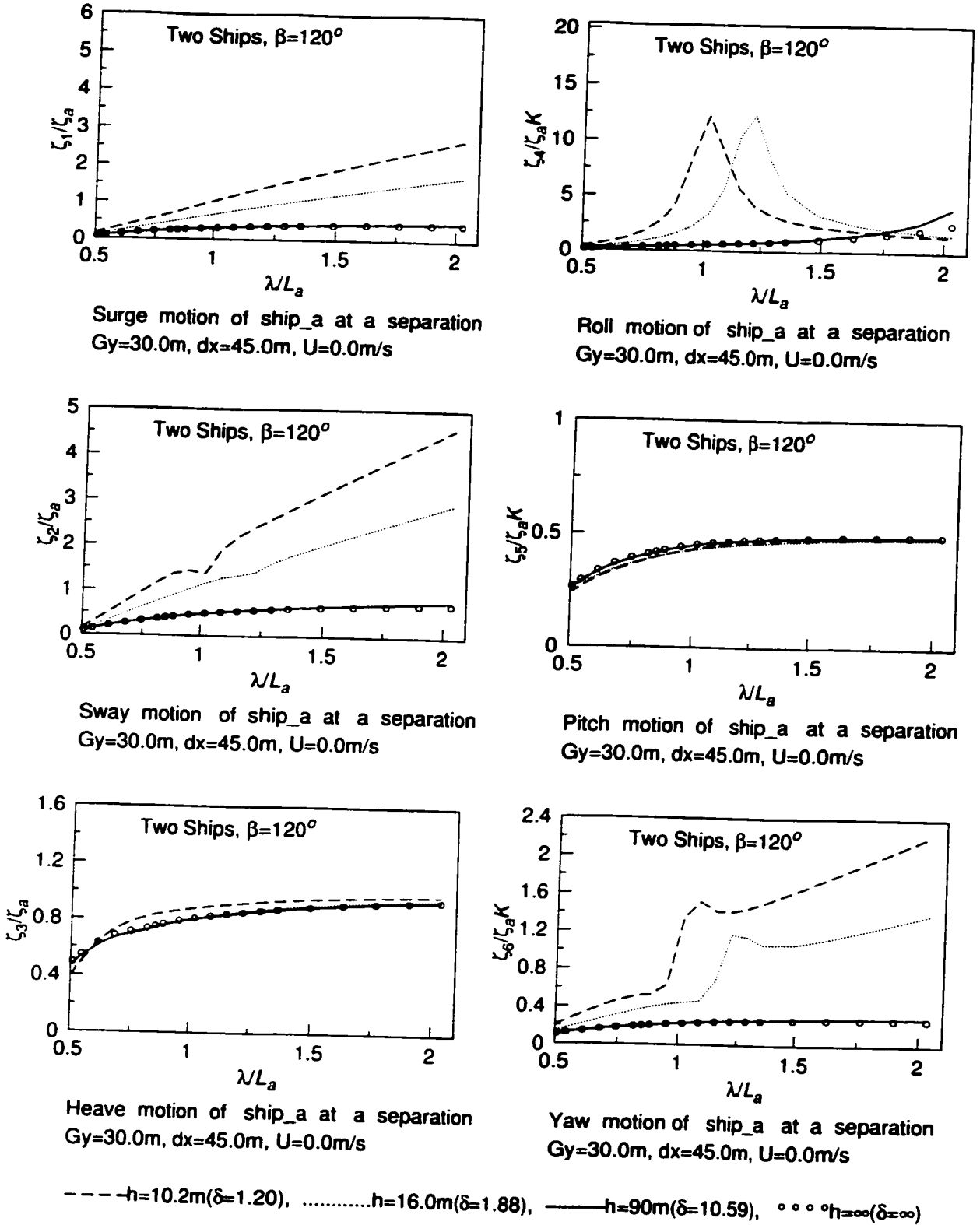
Figure 5.83: Non-dimensional motion displacement amplitudes on ship_a in Case 8
