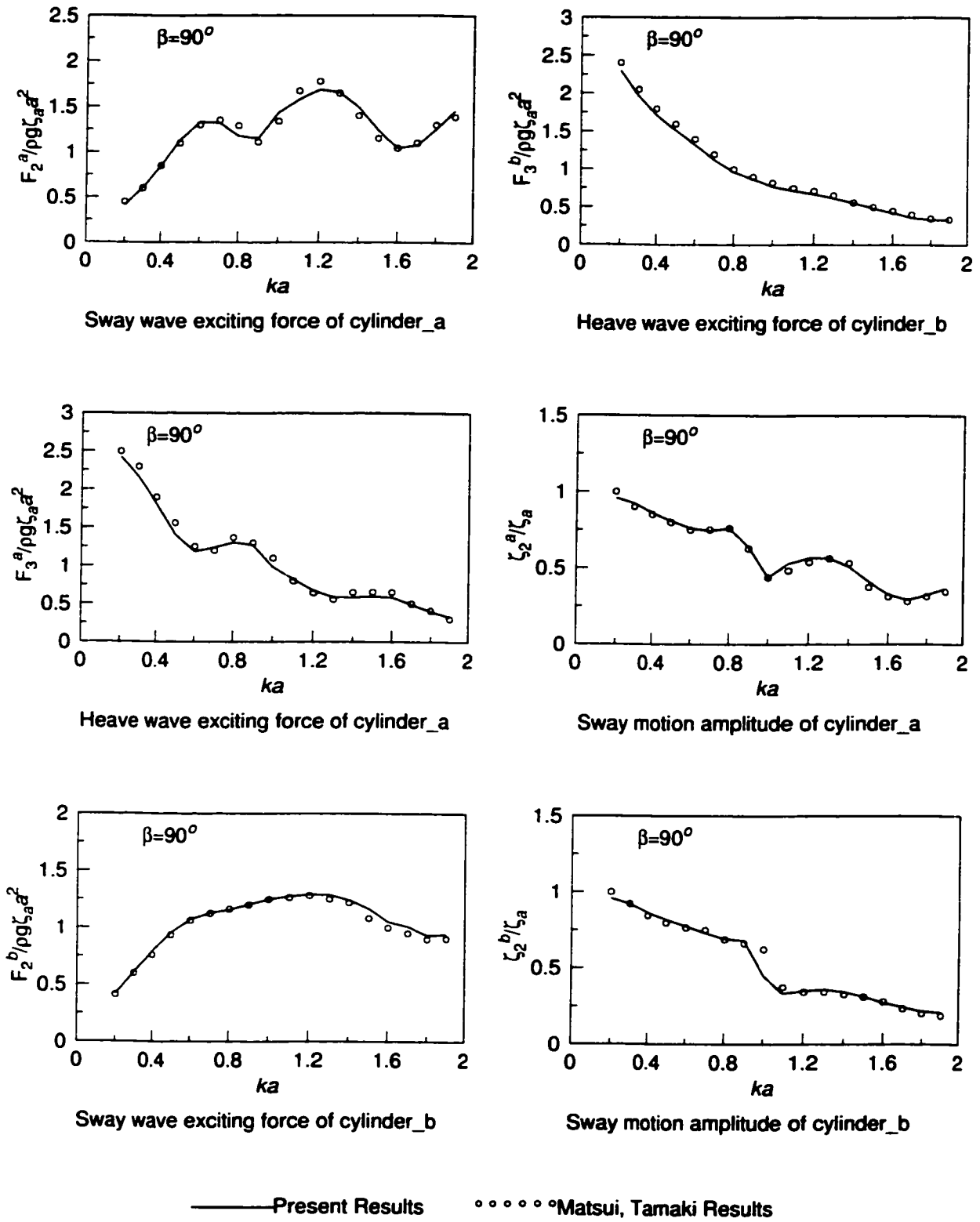
Figure 5.4: Non-dimensional wave exciting forces and motions in test case 1
