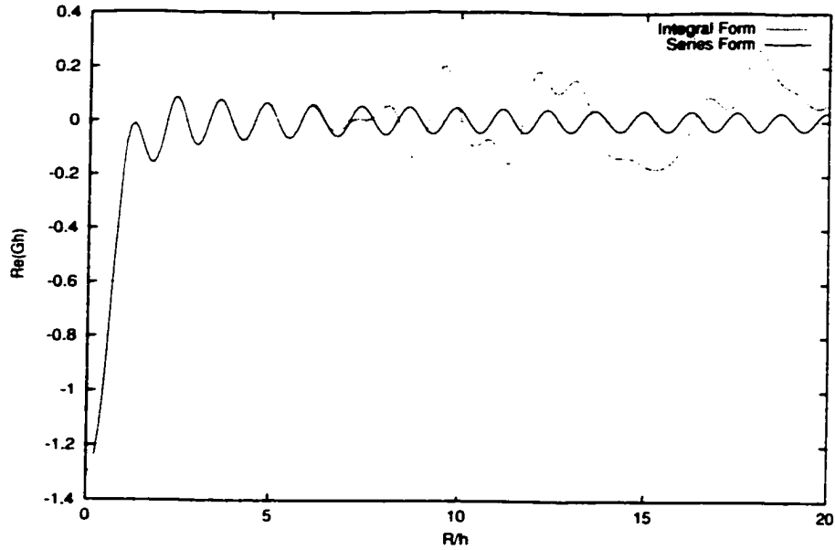
Figure 3.3: Comparison between real part of the integral and series forms of Gh when Kh = 5.0 , kh = 5.000454 , and 0 < R/h < 20
