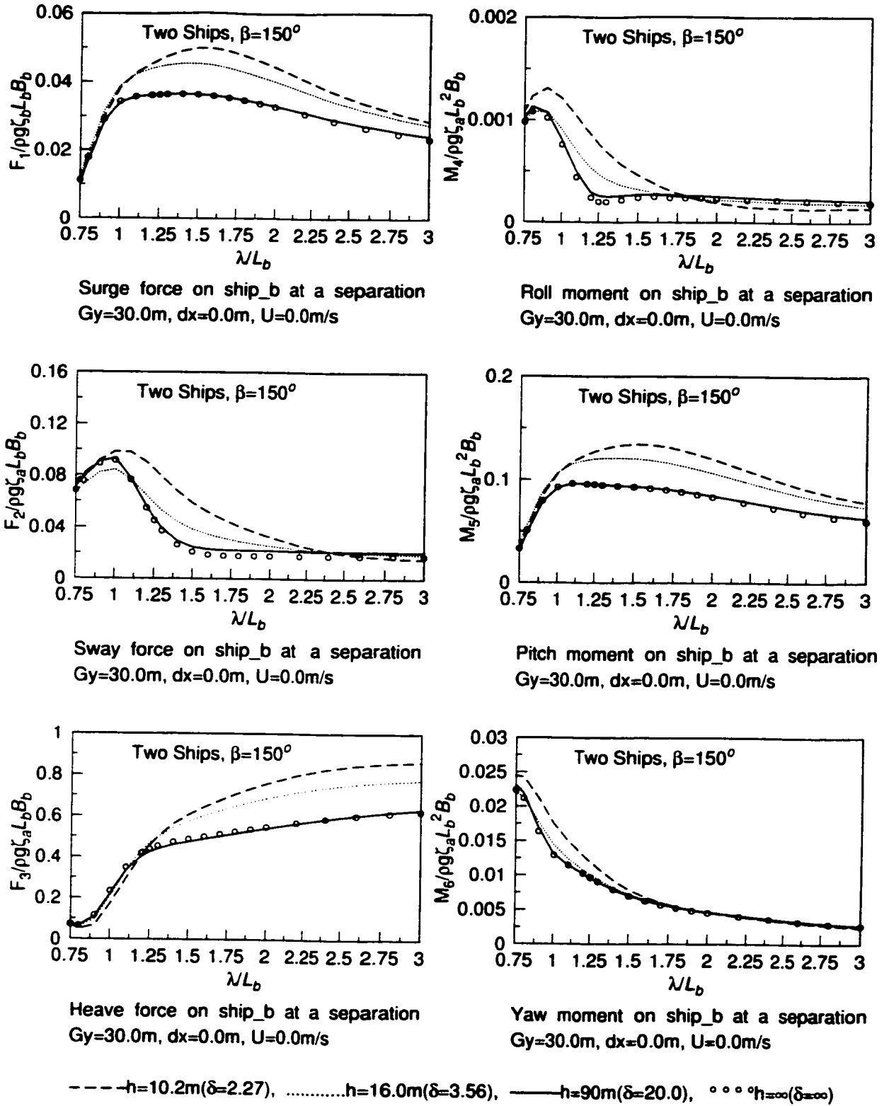
Figure 5.58: Non-dimensional wave exciting force amplitudes on ship_b in Case 5
