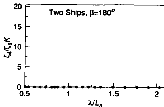
Roll motion of ship_a at a separation Gy=30.0m, dx=45.0m, U=0.0m/s
