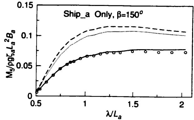
Pitch moment on ship_a at a separation Gy=2000.0m, dx=0.0m, U=0.0m/s
