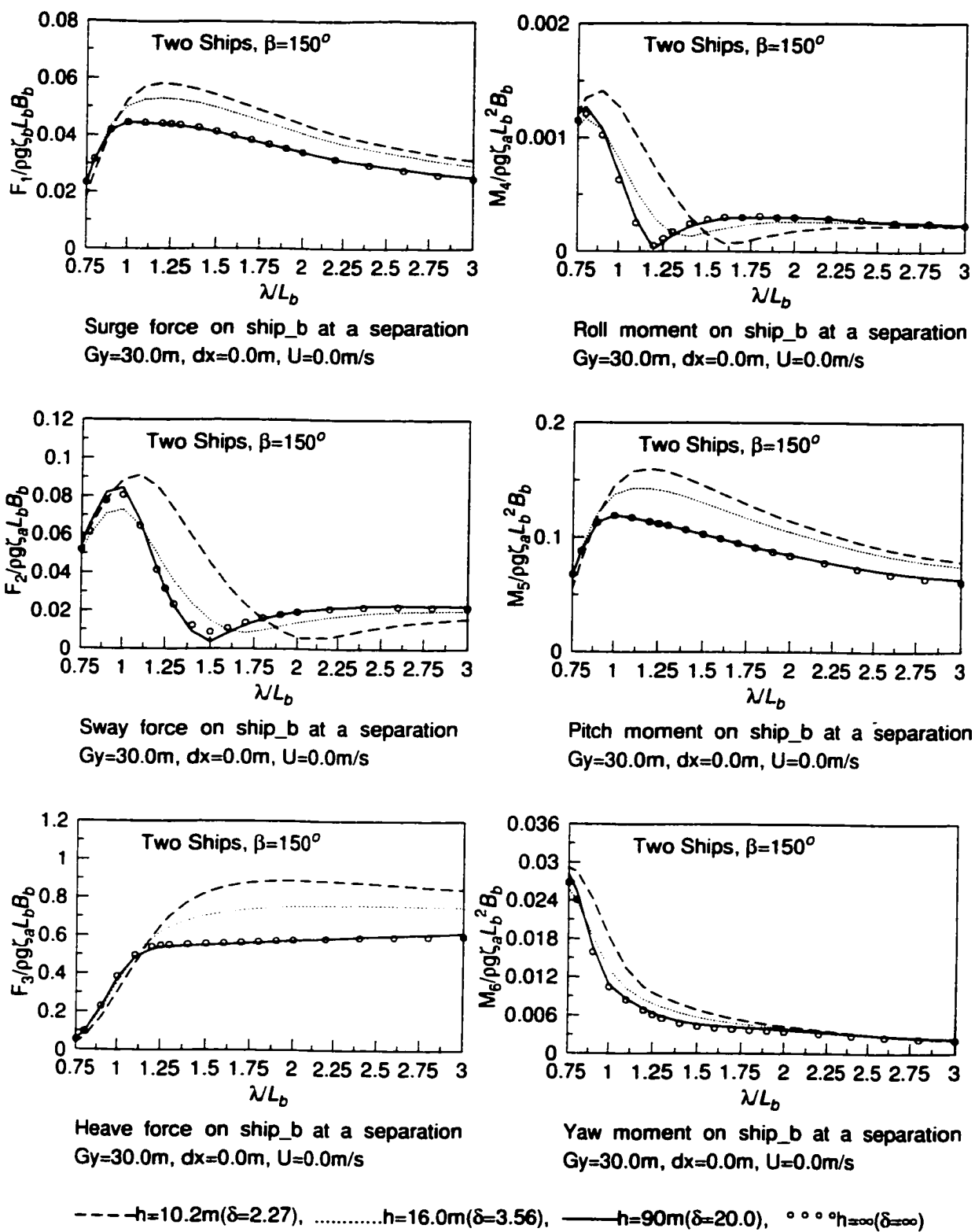
Figure 5.50: Non-dimensional wave exciting force amplitudes on ship_b in Case 4
