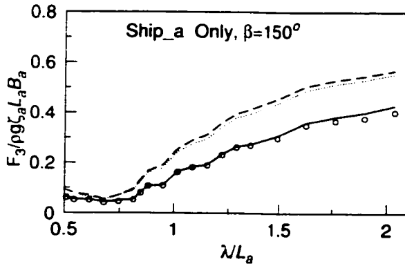
Heave force on ship_a at a separation Gy=2000.0m, dx=0.0m, U=0.0m/s
