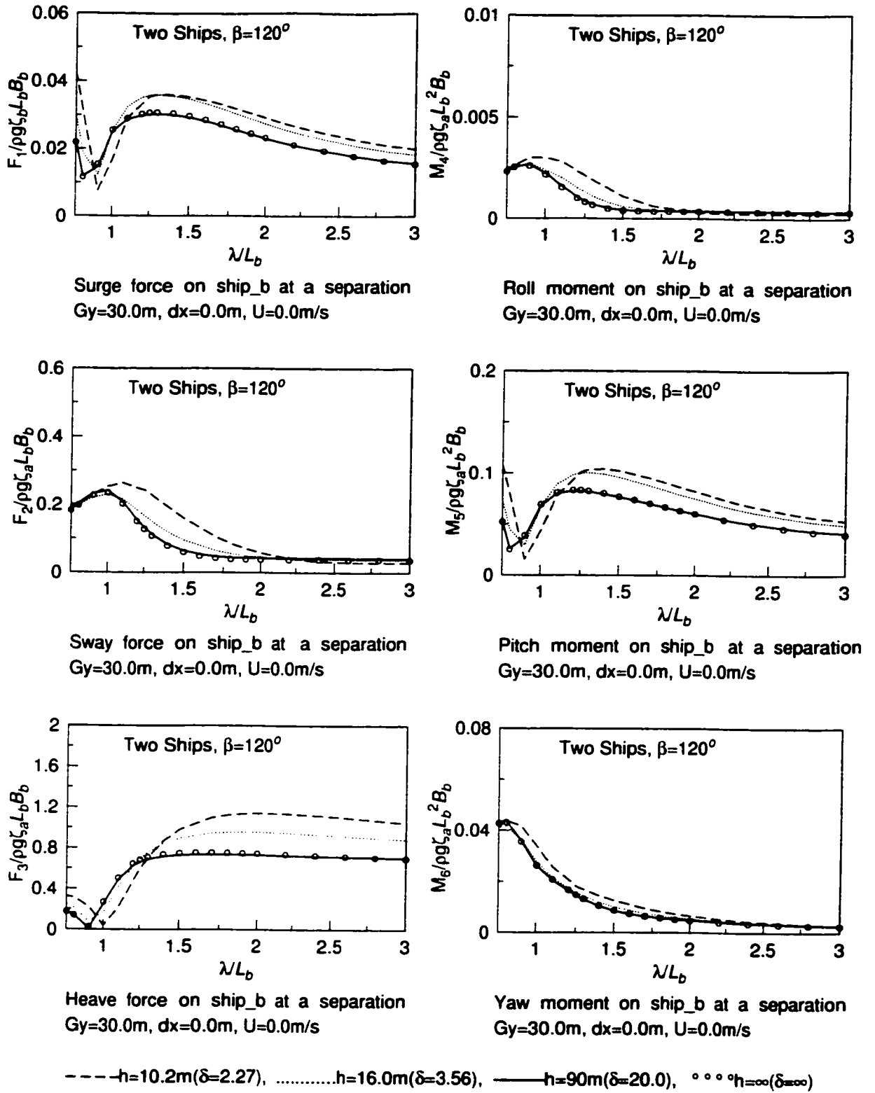
Figure 5.74: Non-dimensional wave exciting force amplitudes on ship_b in Case 7
