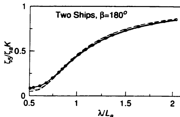
Pitch motion of ship_a at a separation Gy=30.0m, dx=45.0m, U=0.0m/s
