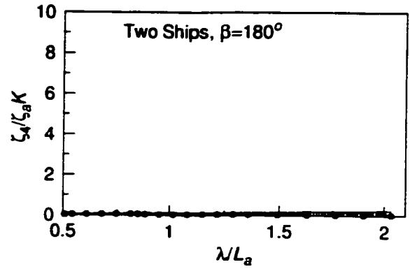
Roll motion of ship_a at a separation Gy=30.0m, dx=45.0m, U=6.18m/s
