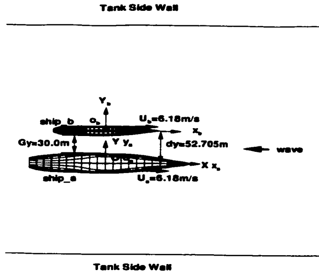
Figure 5.17: Ship_b alongside ship_a, head seas
