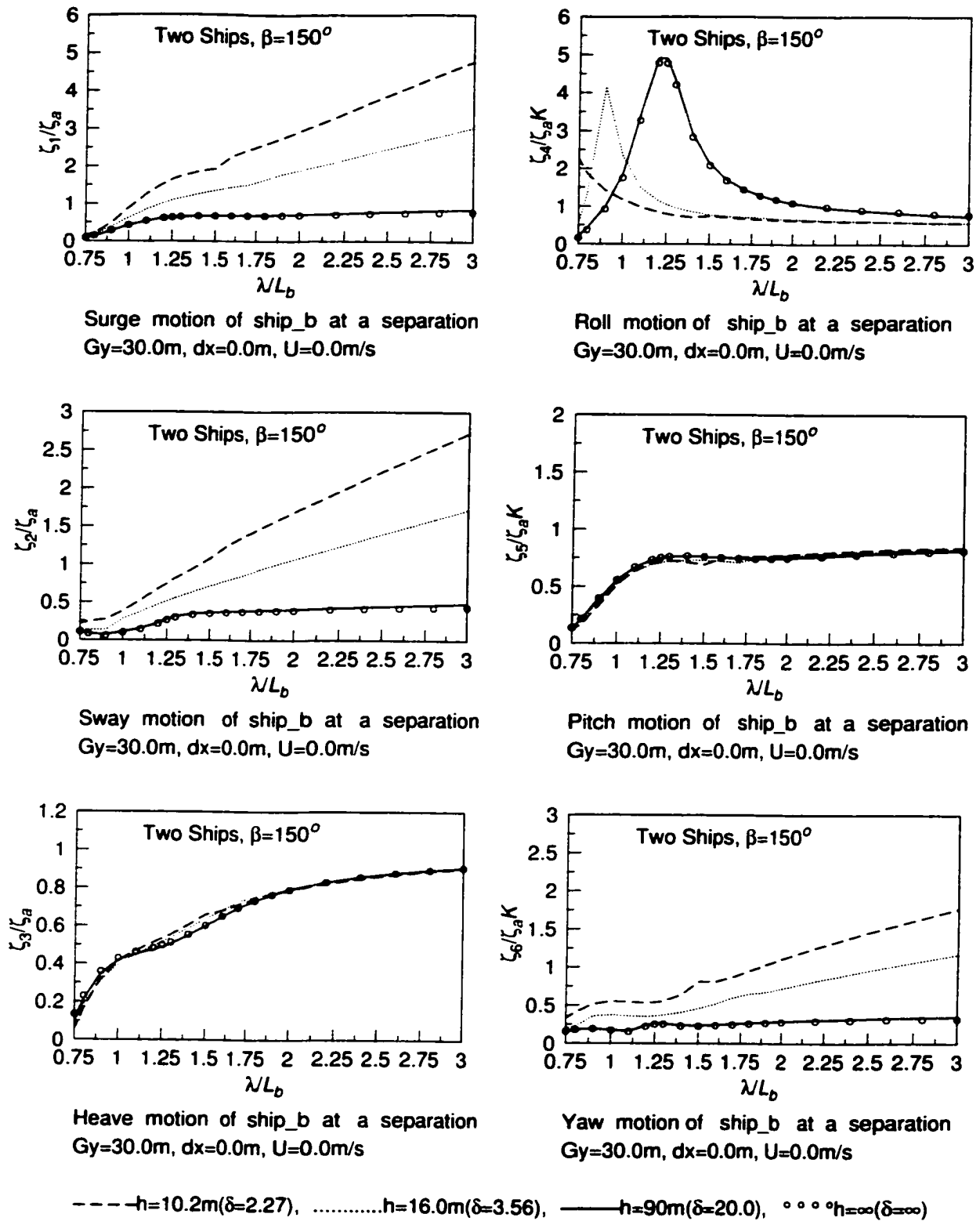
Figure 5.60: Non-dimensional motion displacement amplitudes on ship_b in Case 5
