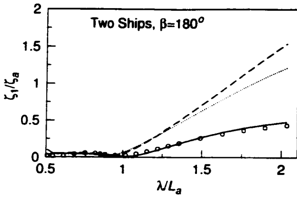
Surge motion of ship_a at a separation Gy=30.0m, dx=45.0m, U=6.18m/s
