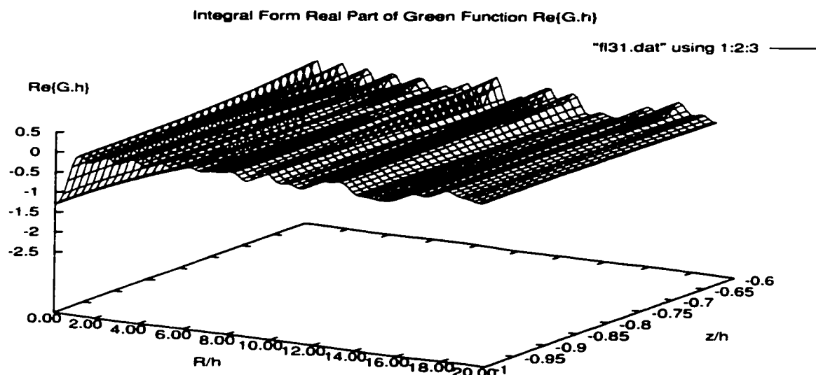
Figure 3.13: The 3-D distribution of the real part of Gh with the integral form when Kh = 5.0 , kh = 5.000454 , and 0 < R/h < 20
