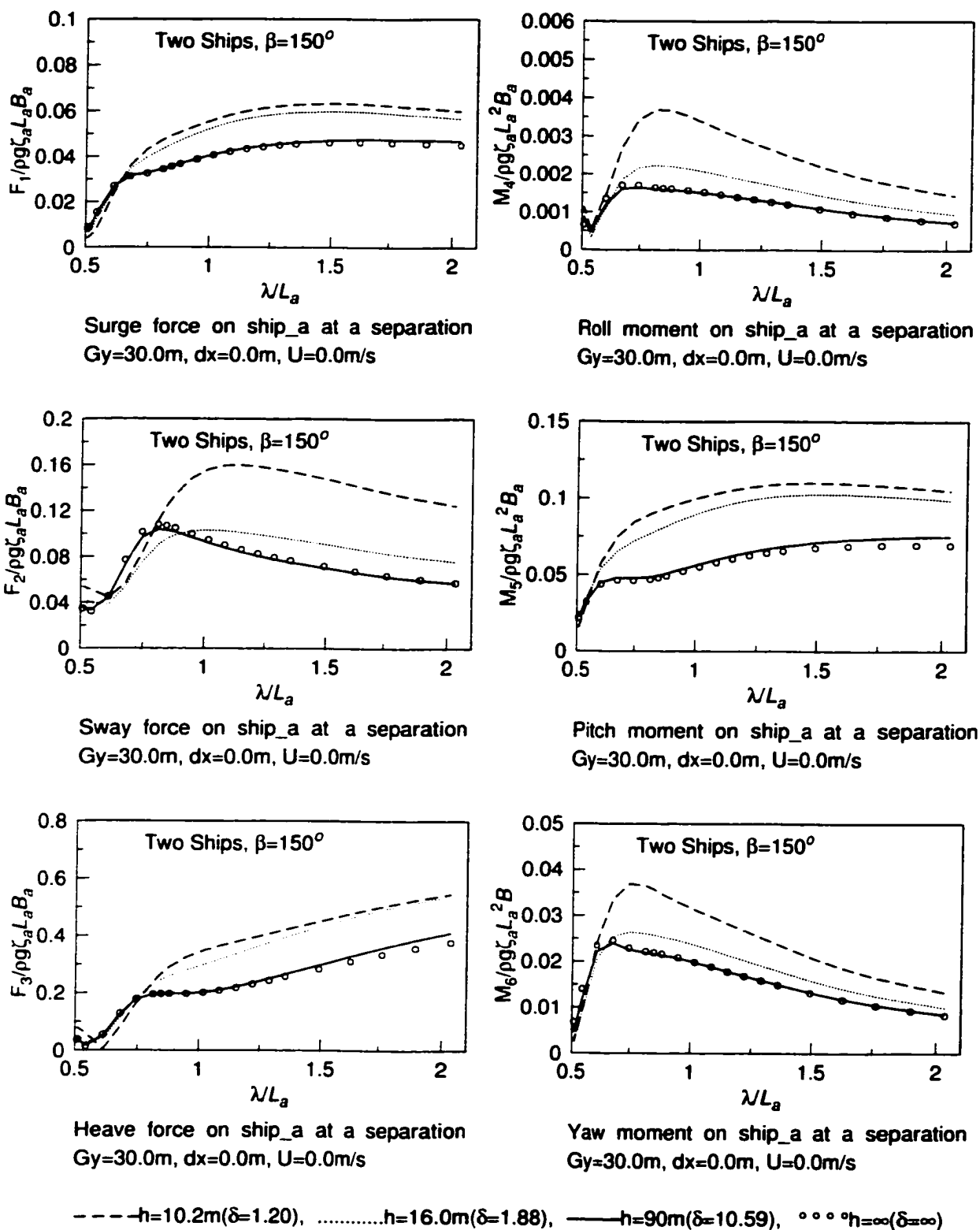
Figure 5.49: Non-dimensional wave exciting force amplitudes on ship_a in Case 4
