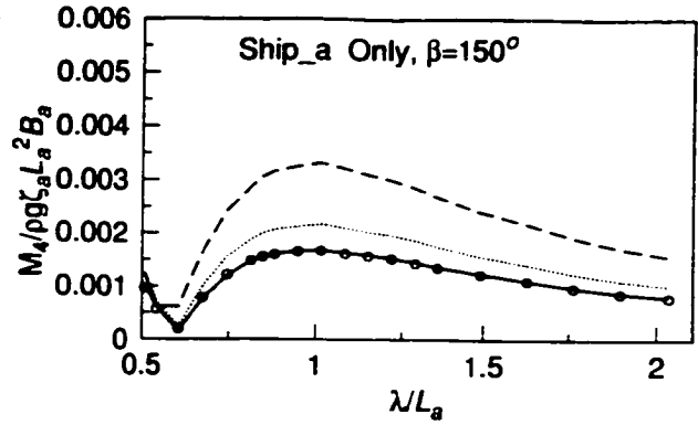
Roll moment on ship_a at a separation Gy=2000.0m, dx=0.0m, U=0.0m/s
