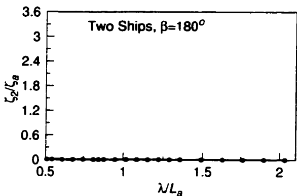
Sway motion of ship_a at a separation Gy=30.0m, dx=45.0m, U=0.0m/s
