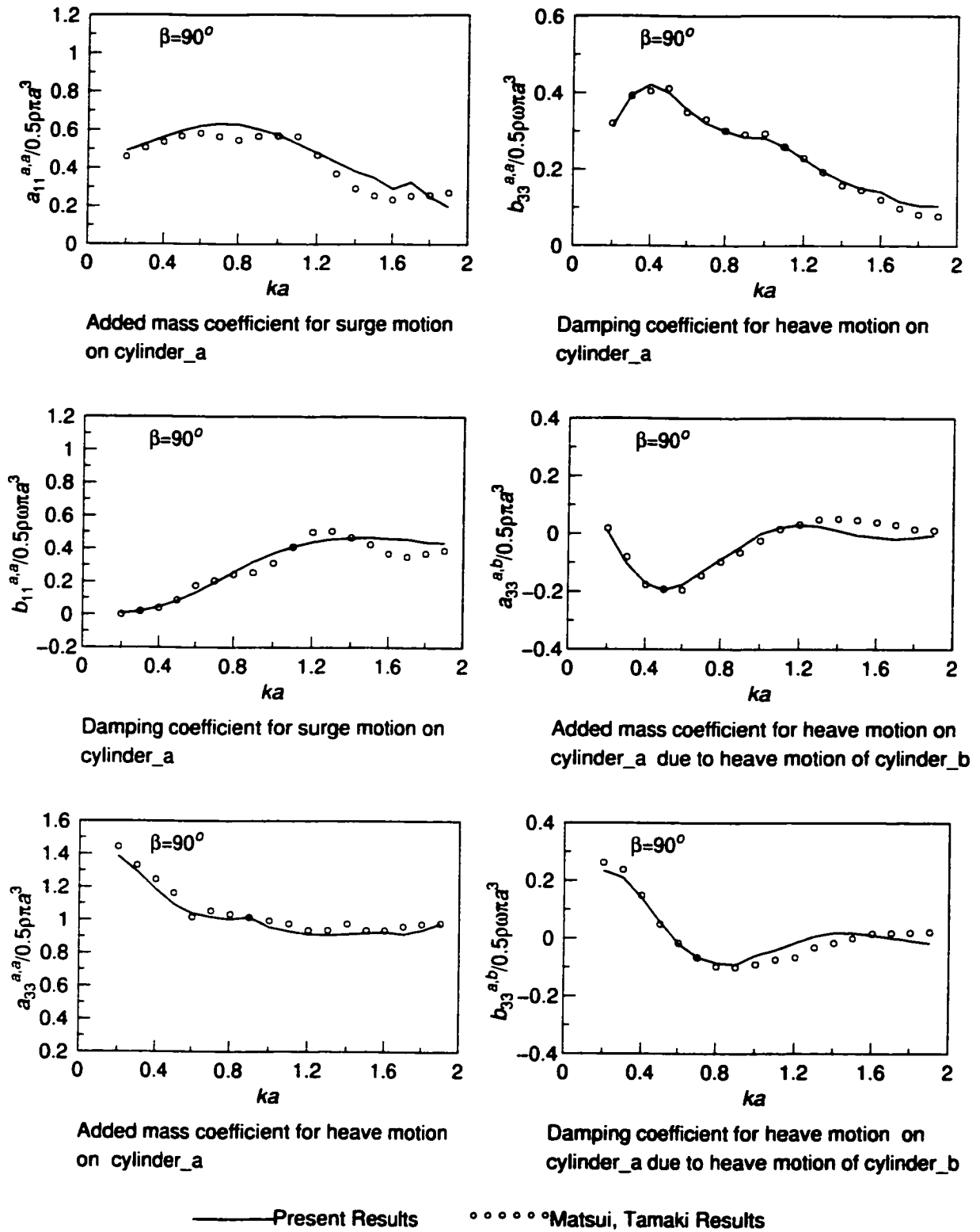
Figure 5.10: Non-dimensional added mass and damping coefficient in test case 2
