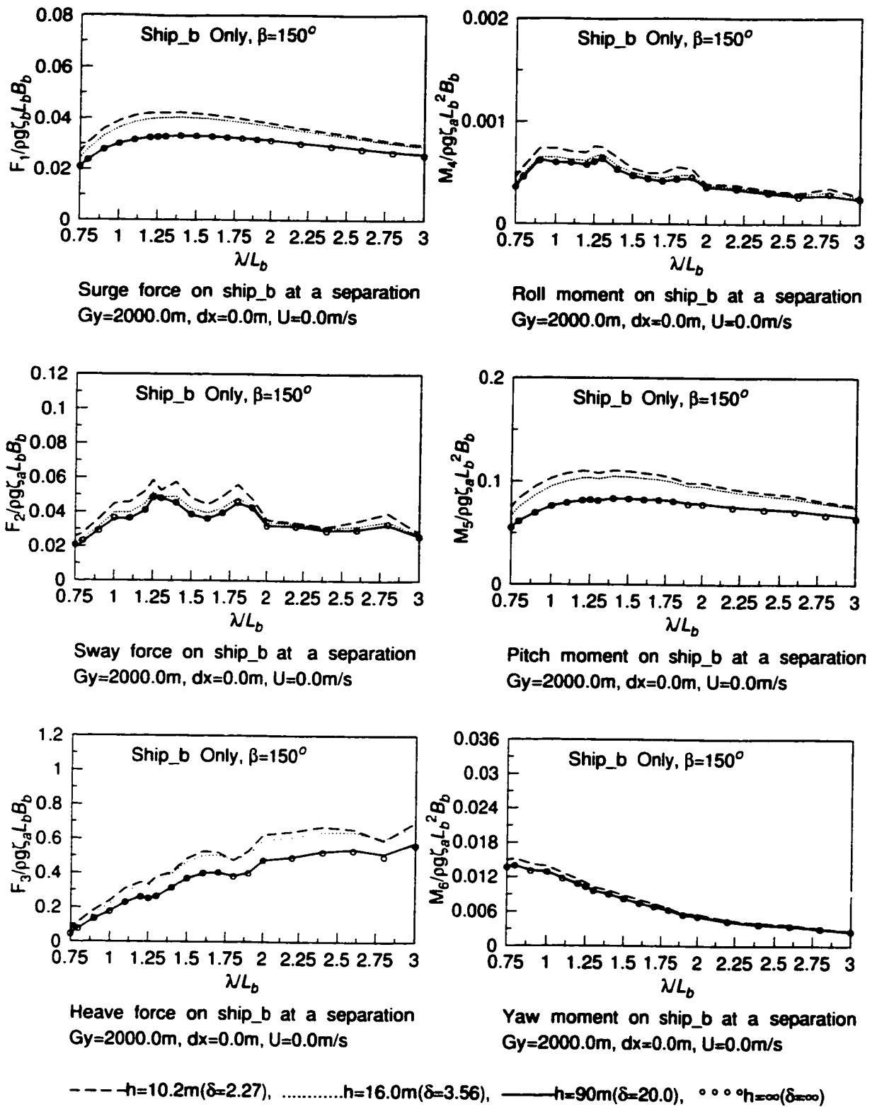
Figure 5.66: Non-dimensional wave exciting force amplitudes on ship_b in Case 6
