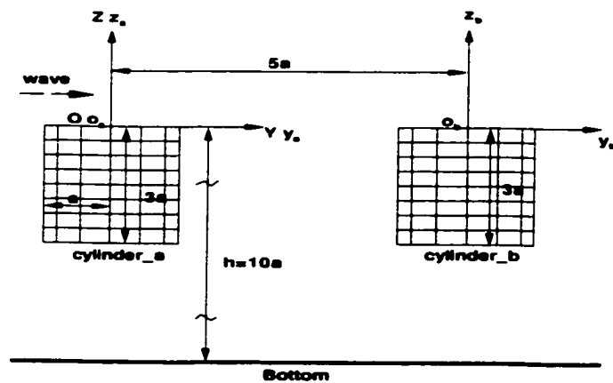
Figure 5.8: Water depth h=10a for test case 2
