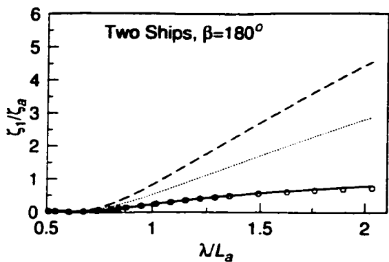
Surge motion of ship_a at a separation Gy=30.0m, dx=45.0m, U=0.0m/s
