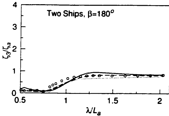
Heave motion of ship_a at a separation Gy=30.0m, dx=45.0m, U=6.18m/s
