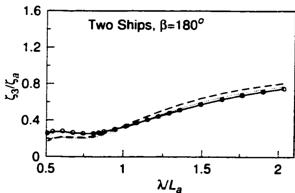
Heave motion of ship_a at a separation Gy=30.0m, dx=45.0m, U=0.0m/s
