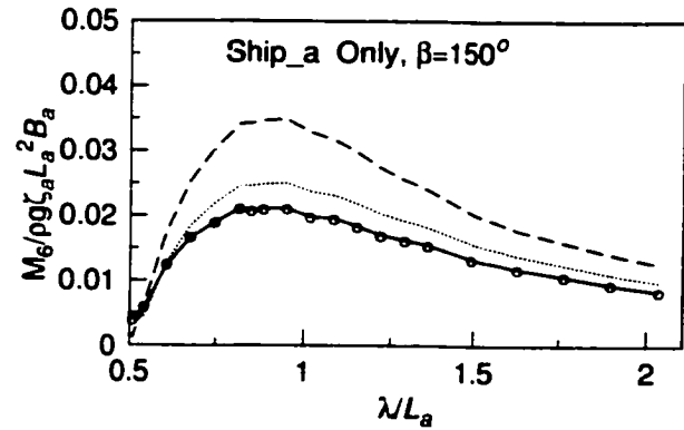
Yaw moment on ship_a at a separation Gy=2000.0m, dx=0.0m, U=0.0m/s
