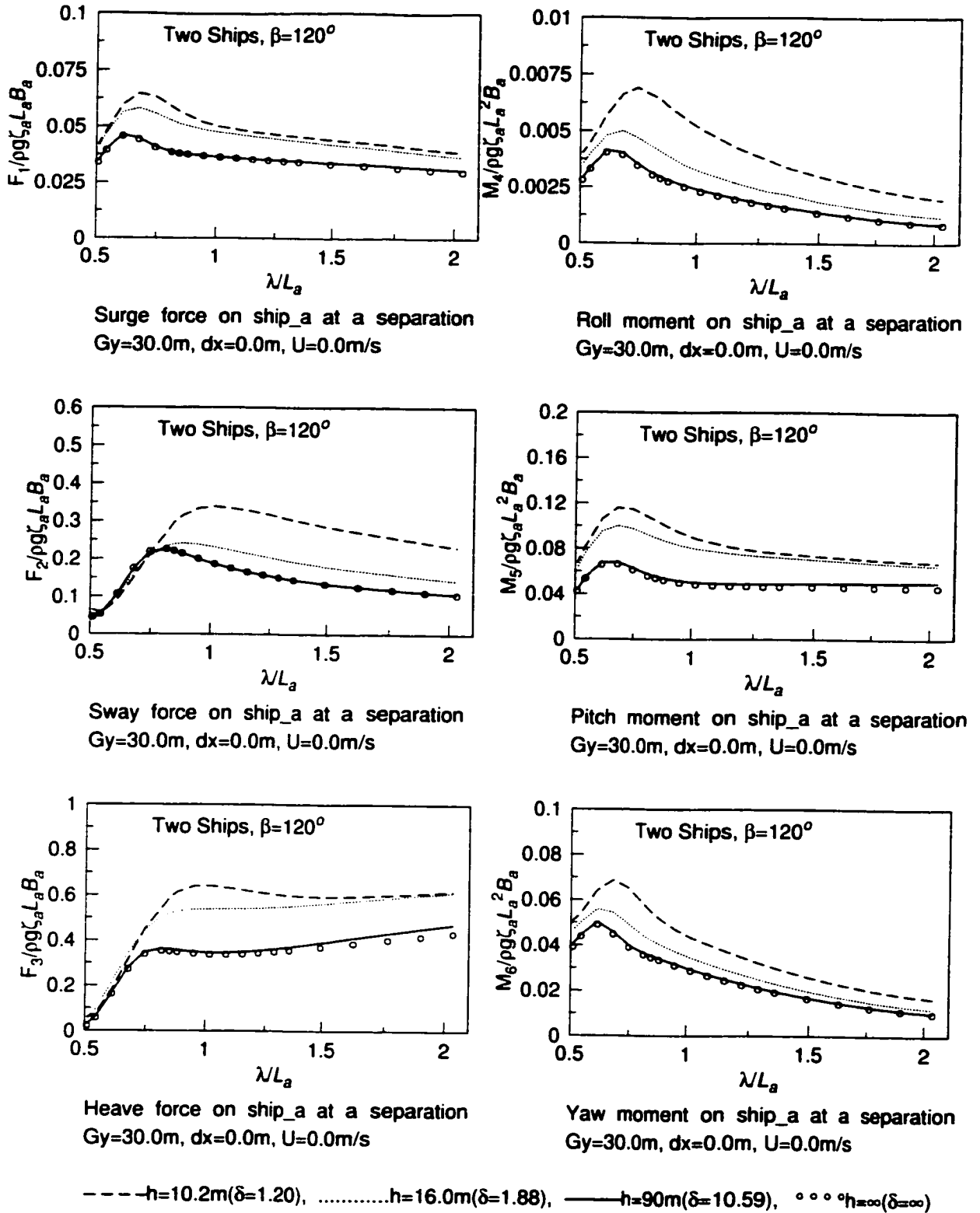
Figure 5.73: Non-dimensional wave exciting force amplitudes on ship_a in Case 7
