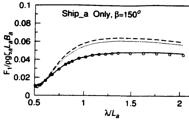
Surge force on ship_a at a separation Gy=2000.0m, dx=0.0m, U=0.0m/s
