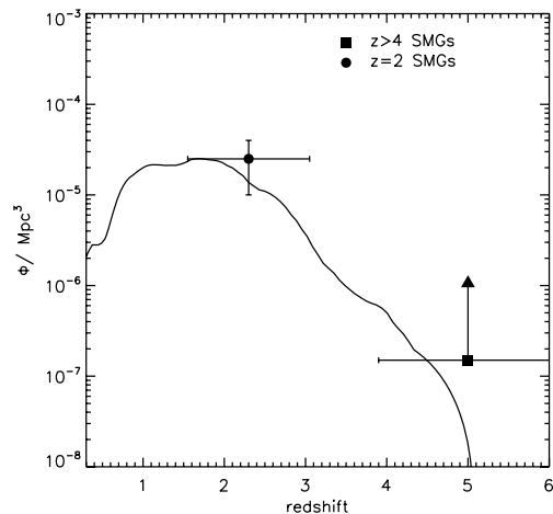
Figure 4. A comparison of the volume density of radio-detected SMGs with S_{1.4\text{GHz}} > 30 \mu\text{Jy} and S_{850\mu\text{m}} > 5 \text{ mJy} from the GALFORM model of Baugh et al. (2005) to our limit on the volume density of z > 4 SMGs and the measured density of z \sim 2 SMGs from Chapman et al. (2005). This demonstrates that these detailed theoretical models are just consistent with these current observations, and so the discovery of more examples of z > 4 SMGs within the ECDF-S would result in a disagreement with the model predictions.
