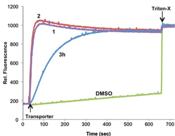
Fig. 3 Anion exchange assay for the natural product prodigiosin 1 relative to synthetic analogues 2 and 3h . Anion exchange from EYPC liposomes was monitored by a change in the fluorescence of lucigenin at 25 °C after addition of 0.04 mol% of prodigiosene transporter relative to EYPC lipid. The EYPC liposomes, containing 1 mM lucigenin, 20 mM HEPES buffer (pH 7.43) and 100 mM NaCl were suspended in a solution of 20 mM HEPES buffer (pH 7.43) that contained 100 mM NaNO 3 . At t = 30 s, the prodigiosene transporter was added and the fluorescence of lucigenin was monitored ( \lambda_{\text{ex}} = 372 nm, \lambda_{\text{em}} = 504 nm). At t = 660 s, the addition of triton-X lysed the liposomes.
