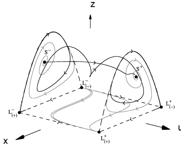
FIG. 2. Phase diagram of the system (10)–(12) for \Lambda < 0 and \Lambda_M > 0 , where \phi > 0 is assumed. See caption to Fig. 1. Gray lines represent typical trajectories found within the two-dimensional invariant sets, dashed black lines are those trajectories along the intersection of the invariant sets, and solid black lines are typical trajectories within the full three-dimensional phase space.
