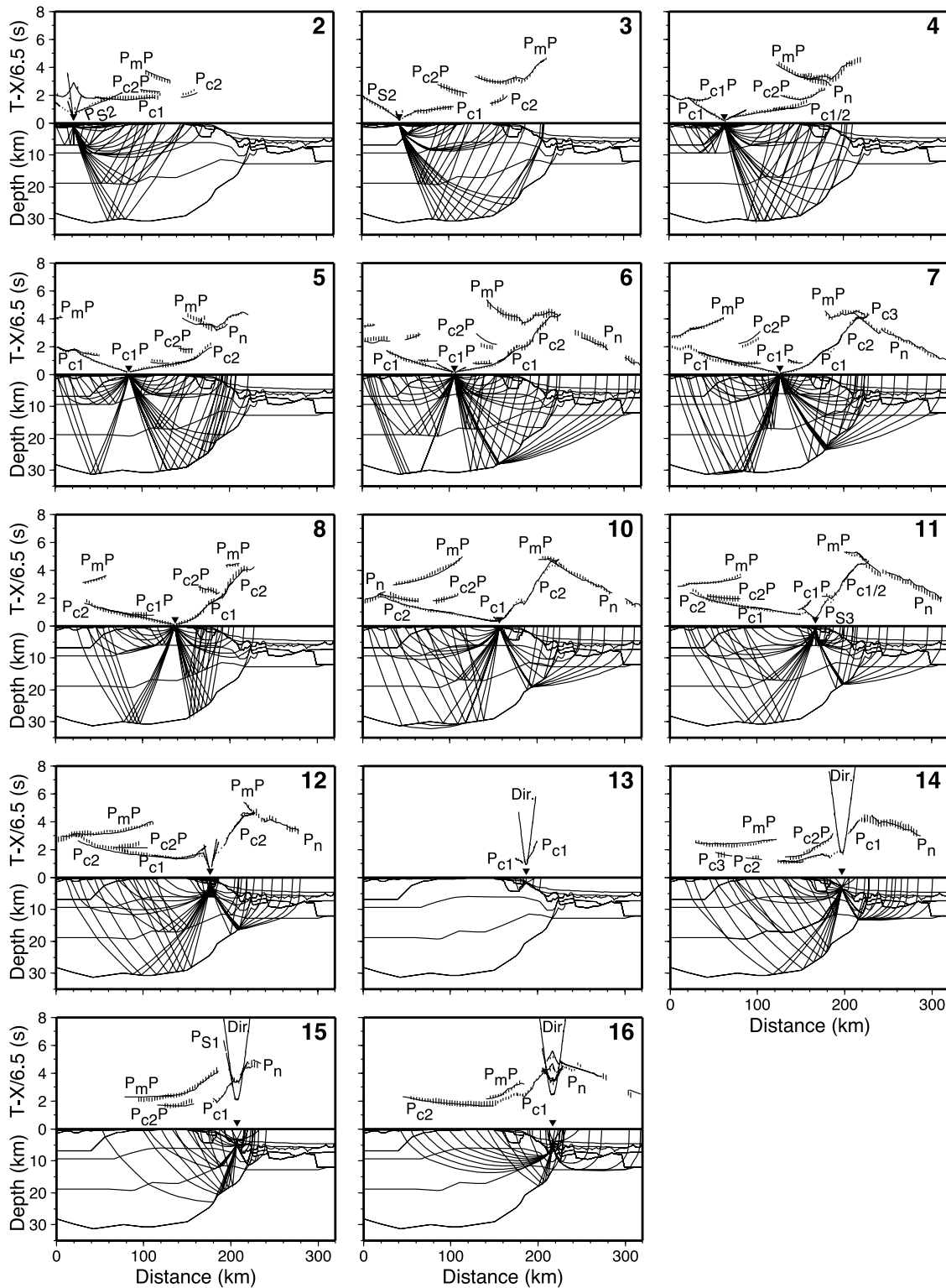
Figure 8. Comparison of observed and calculated travel times for OBS 2–16, shown together with the corresponding ray paths. Observed data are indicated by vertical bars, with heights representing pick uncertainty; calculated data are indicated by solid lines. Triangles mark the receiver locations. Horizontal scale is the model position; a reduction velocity of 6.5 km/s has been applied for the travel times. Abbreviation Dir. is the direct wave.
