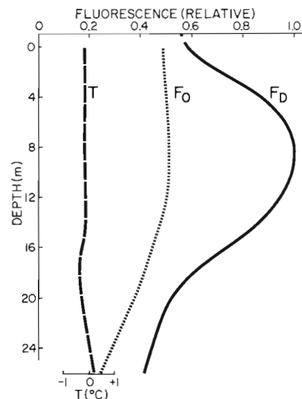
Fig. 8. Depth distribution of fluorescence ( F_0 -without DCMU; F_D -with DCMU) and temperature on 1 d during spring bloom. 16 March was characterized by winds in excess of 20 \text{ m s}^{-1} with a correspondingly high rate of energy dissipation measured with a microscale velocity profiler
