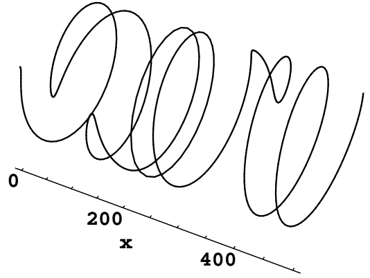
FIG. 1. A section of a system from a simulation using non-conserved dynamics. Distance along the system is shown by the scale and the unit-magnitude order parameter is shown in the orthogonal plane. The windings of \pm 2\pi (textures/anti-textures) of scale L_w and the clusters of monotonic winding of a larger scale L are evident.
