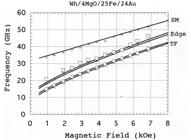
FIG. 11. Frequencies vs applied magnetic field for the composite specimen Fe-whisker/4 ML MgO/25 ML Fe/24 ML Au(001). TF, thin-film frequencies; \circ , upshifted frequencies; \times , downshifted frequencies. SM, iron whisker surface mode frequencies. Edge-bulk iron manifold edge frequencies, respectively. The solid lines were calculated for zero exchange coupling using following parameters: (1) Thin film: 4\pi M_s = 21.4 kG, g = 2.09 , perpendicular surface anisotropy K_s = 1.65 erg/cm 2 , in-plane anisotropy parameter K_1 = 4.0 \times 10^5 erg/cm 3 , and thickness d = 3.58 nm. (2) Bulk iron: 4\pi M_s = 21.4 kG, g = 2.09 , exchange stiffness A = 2.03 \times 10^{-6} erg/cm, perpendicular surface anisotropy K_s = 1.0 erg/cm 2 , and in-plane anisotropy parameter K_1 = 4.76 \times 10^5 erg/cm 3 .
