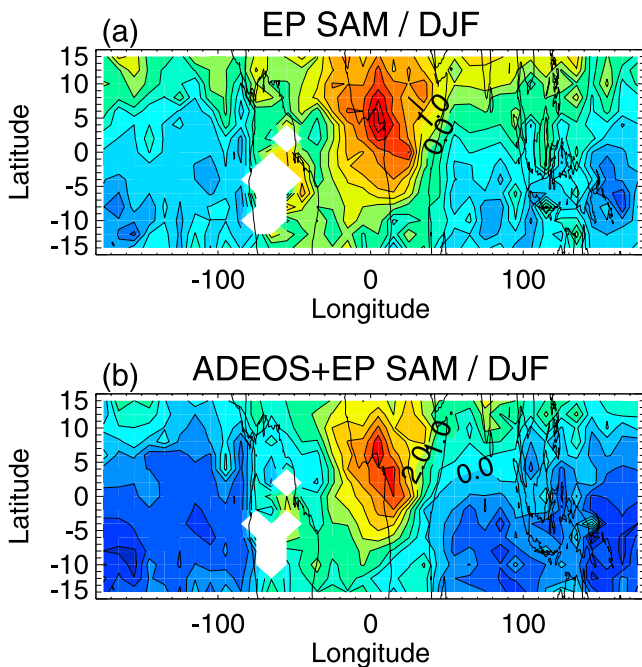
Figure 3. Distribution of tropospheric ozone index derived from (a) the EP-only SAM and (b) the ADEOS + EP SAM for December 1996 to February 1997.
