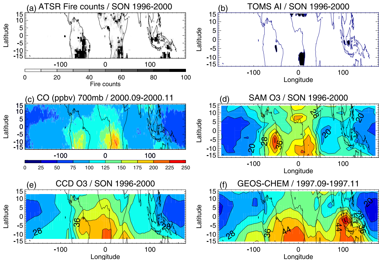
Figure 7. As in Figure 4, but in the September–October–November time period.
