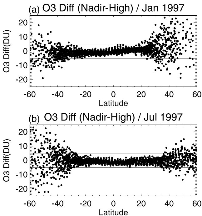
Figure 1. Latitudinal variation of the total ozone difference between nadir and high-scan positions in (a) January and (b) July 1997.
