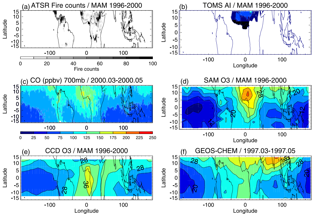
Figure 5. As in Figure 4, but in the March-April-May time period.
