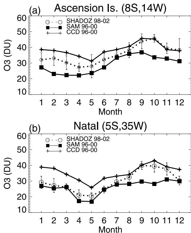
Figure 8. Monthly mean tropospheric ozone column (DU) from SAM (solid squares), the CCD method (crosses), and the SHADOZ measurements (open circles) at (a) Ascension Island (8°S, 14°W) and (b) Natal (5°S, 35°W).
