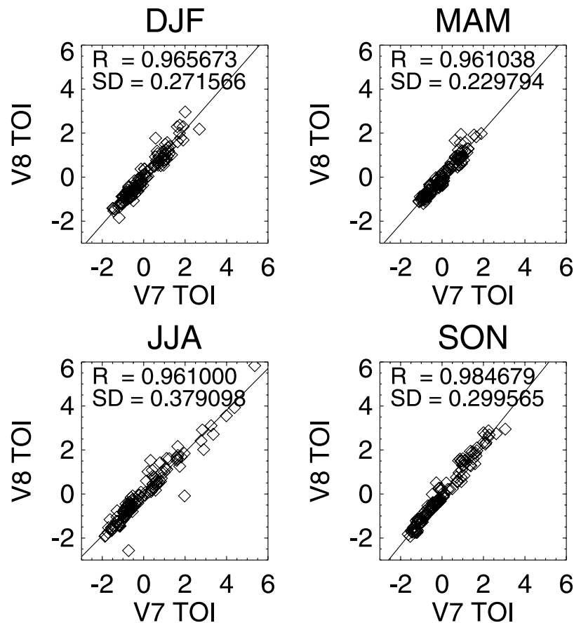
Figure 10. Comparison of tropospheric ozone index (TOI) residuals, which are the TOI values subtracted from zonal mean, from version 7 and version 8 TOMS data in four seasons. The R and SD represent the regression coefficient and standard deviation (one-sigma level).
