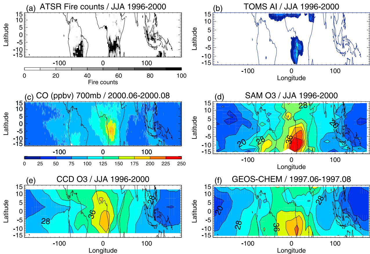
Figure 6. As in Figure 4, but in the June-July-August time period.
