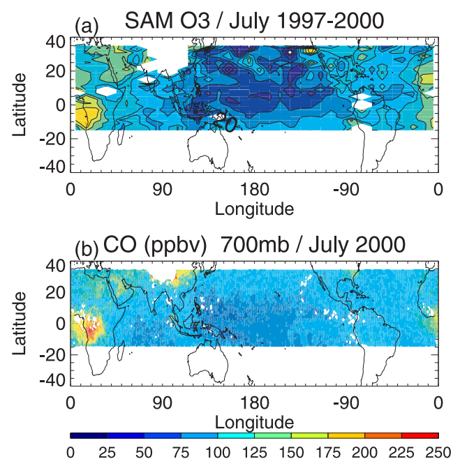
Figure 2. Distribution of (a) tropospheric ozone column (DU) derived from SAM for July from 1997 to 2000 and (b) CO measured from MOPITT for July 2000. White space between 15^\circ\text{S} and 35^\circ\text{N} shows cloudy regions.
