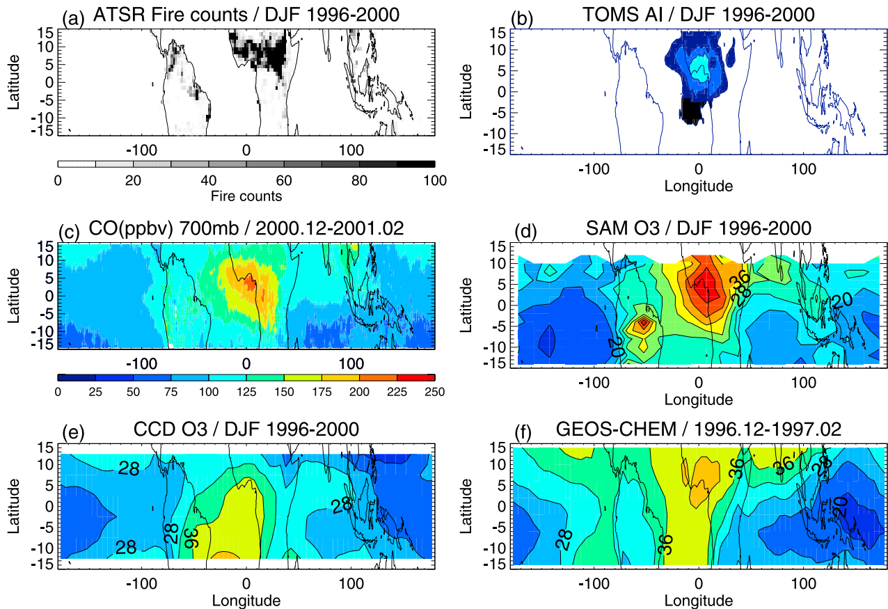
Figure 4. Distribution of (a) fire counts from ATSR averaged for 1996–2000, (b) aerosol index from TOMS averaged for 1996–2000, (c) CO from MOPITT for 2000, (d) tropospheric ozone column (DU) from SAM averaged for 1996–2000, (e) tropospheric ozone column (DU) from CCD averaged for 1996–2000, and (f) tropospheric ozone column (DU) from GEOS-CHEM model for 1997 in the December–January–February time period.
