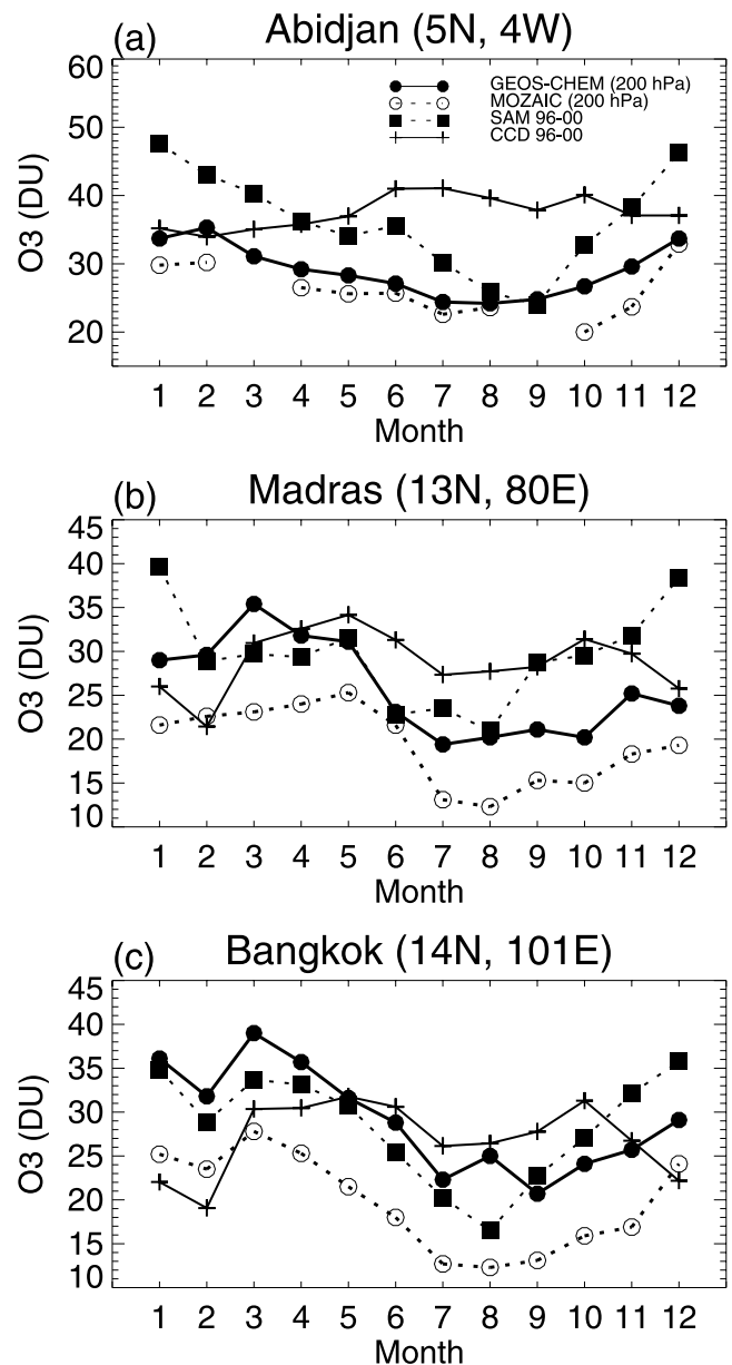
Figure 9. Monthly mean tropospheric ozone column (DU) from SAM (solid squares), the CCD method (crosses), the GEOS-CHEM model (solid circles), and the MOZAIIC observations (open circles) over at (a) Abidjan (5°N, 4°W), (b) Madras (13°N, 80°E), and (c) Bangkok (14°N, 101°E).
