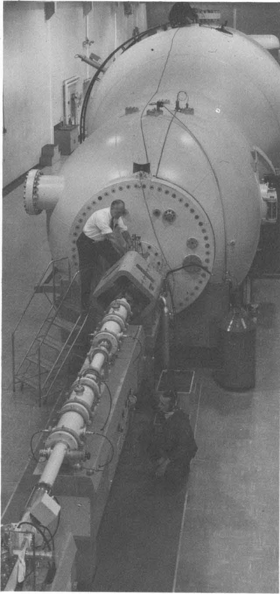
The Tandem Van de Graaff Accelerator at the Chalk River Nuclear Laboratories of Atomic Energy of Canada Limited. Below is a view of the control room.
