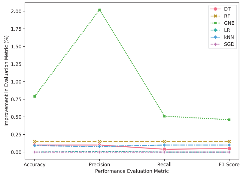
Figure 4.1: Performance Improvement of Traditional ML-based IDS with Selected Features from UNSW-NB15 Dataset
