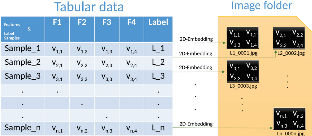
Figure 5.1: Process of Transforming Tabular Data to Images using SuperTML.
