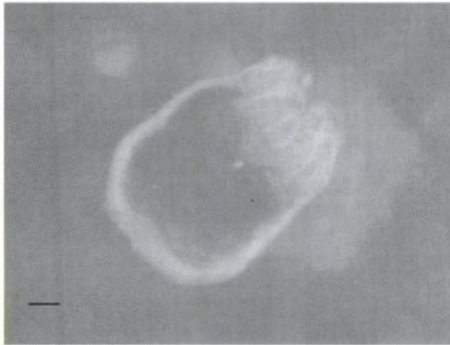
Figure 1. Green hydra contraction and tentacle reduction during the experiment. Bar 500 \mu m.
