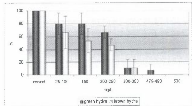
Figure 6. Reaction to mechanical stimuli of green and brown hydra in the experiment (mean \pm s.d).
