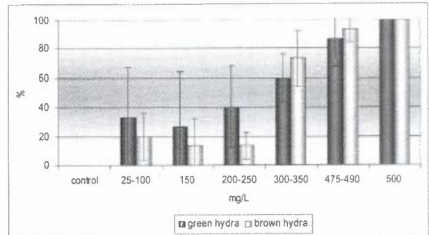
Figure 5. Tentacle reduction of green and brown hydra in the experiment (mean \pm s.d).
