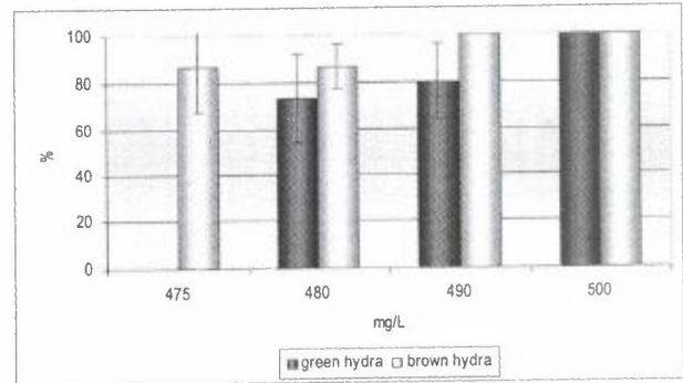
Figure 3. Mortality of green and brown hydra in the experiment (mean \pm s.d).
