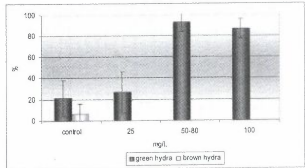
Figure 4. Budding of green and brown hydra in the experiment (mean \pm s.d).
