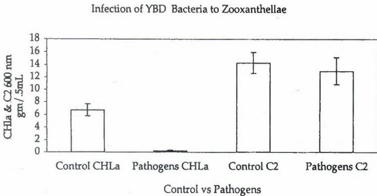
Figure 3: Changes in Chlorophyll a and c2 concentrations in YBD infected corals and controls.
