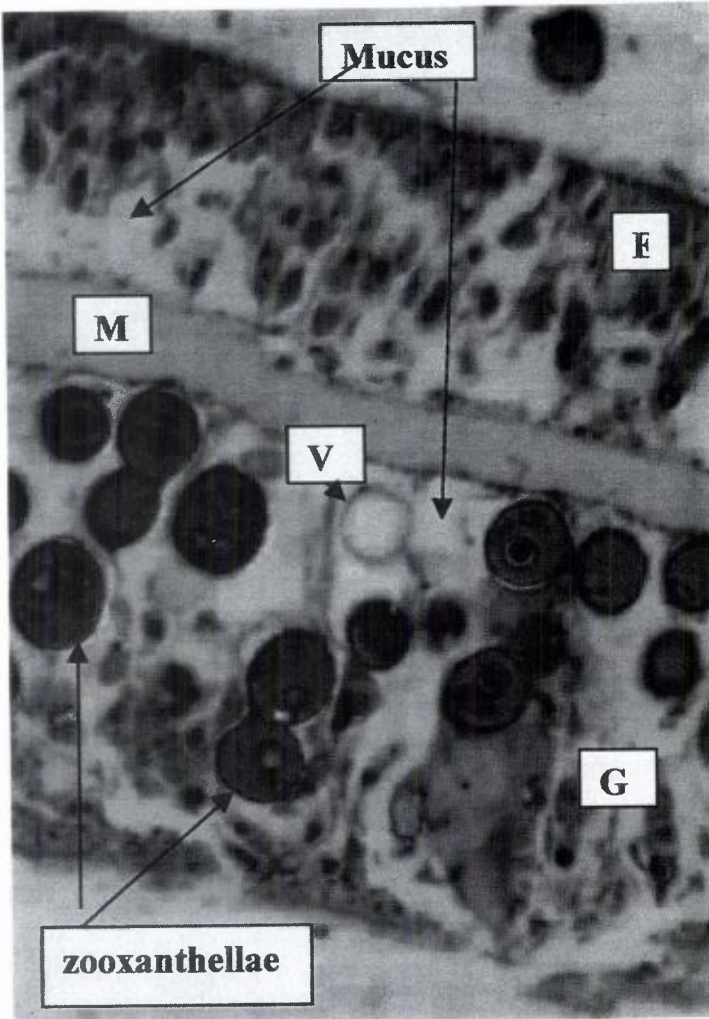
Figure 7. a-b: Histology of Montastraea sp. exposed to YB pathogens at 32°C. Vacuolation and swollen alga can be seen. However, host structural features are evident indicating early breakdown and pockets of copious mucus, however, symbiotic zooxanthellae remain inside the host gastroderm. b: Histological section of healthy Montastraea sp at 25°C, early signs of stress are evident due to a build-up in mucocytes. E=epidermis, V=vacuole, M=mesoglea, G=gastroderm and zoox= symbiotic algae.
