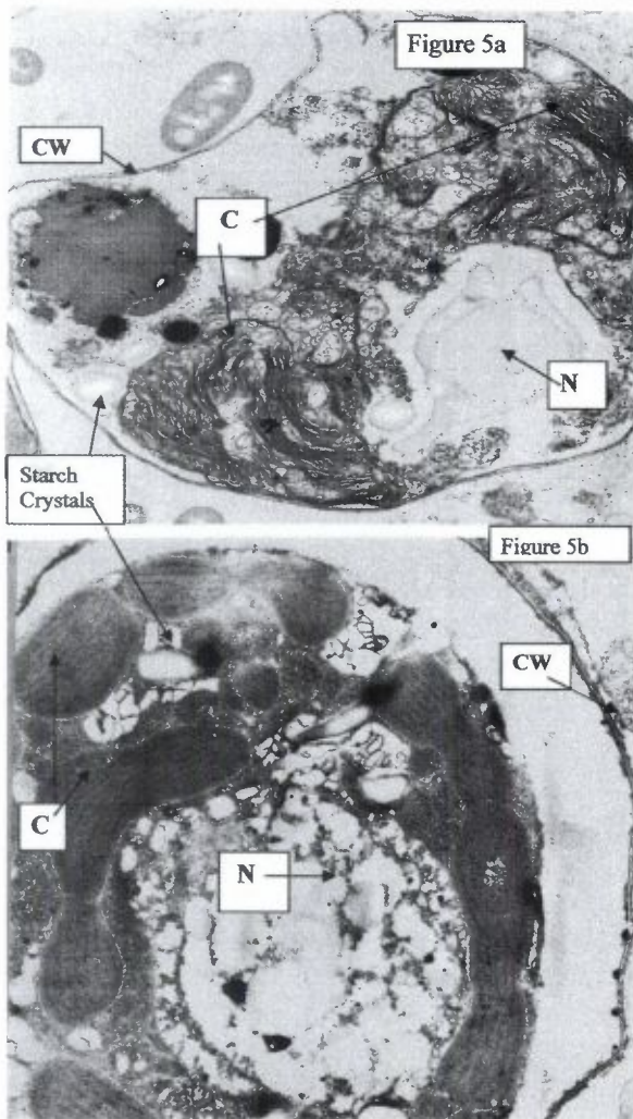
Figure 5. a-b: Shows a transmission electron micrograph (TEM) image of symbiotic exposed to YBD bacteria. TEMs of zooxanthellae in situ indicate the same general morphology as seen in light microscopy, but reveal far greater detail. a: Image shows degradation of cell wall that appears to be evident along with vacuolation and cytoplasmic shrinkage. The chloroplasts are disorganized to the outer margin of the cell; however, they appear intact. There are numerous non-membrane bound vacuoles that appear within the nucleus and cytoplasm of the zooxanthellae. Some of these are filled with an electron dense substance, but many are empty or filled with fluid. b: The core of the algal cells is severely vacuolated. The pyrenoid body is apparent and normal in structure. However, in some cells, the pyrenoid is fragmented into separate segments. Algal swelling is primarily attributable to the expansion of the accumulation bodies separation of the algal surface membranes from the peripheral cytoplasm containing chloroplasts. N=nucleus, C=chloroplasts, S=starch crystals, CW=cell-wall.
