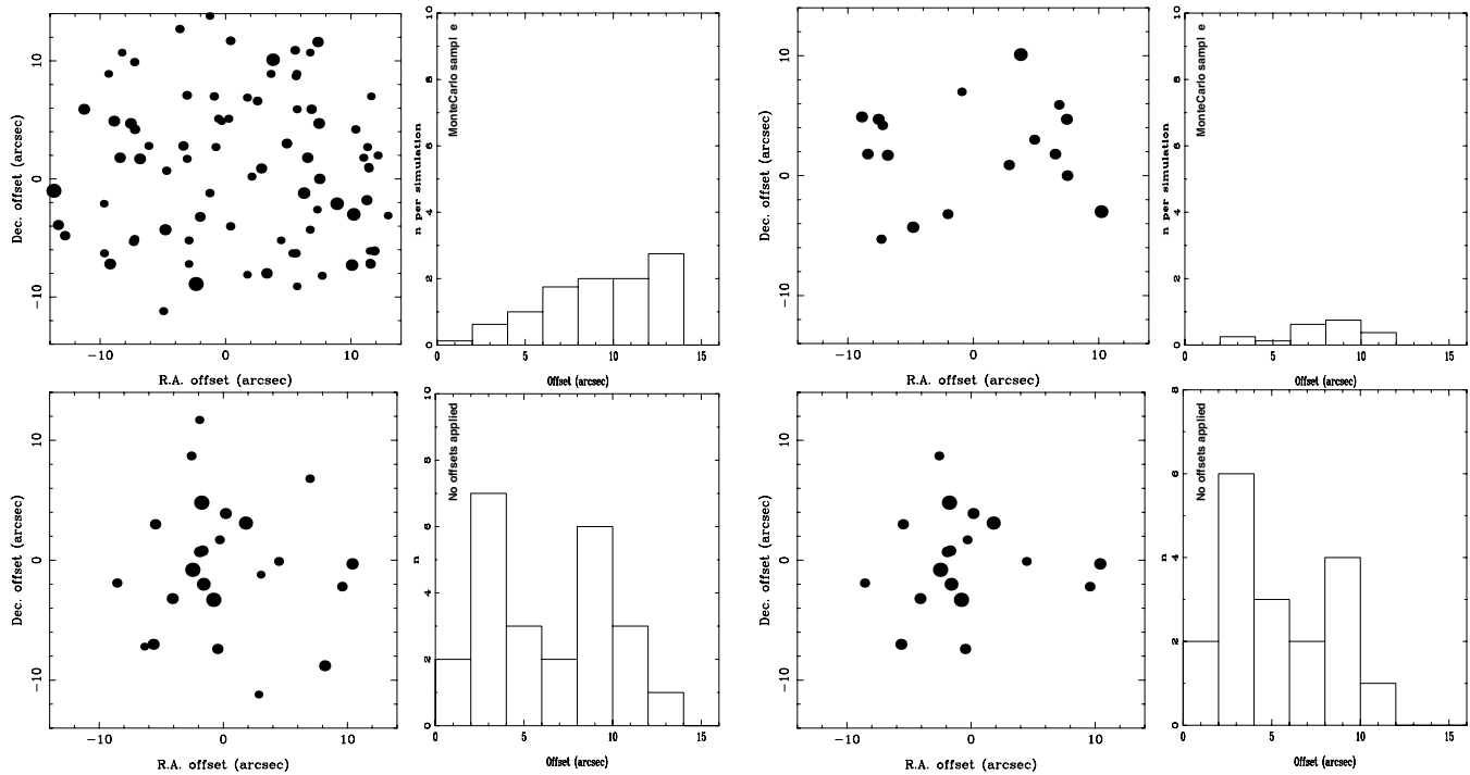
Figure 1. Left-hand panels: positional offsets between SCUBA and MAMBO peaks for spurious (top) and real (bottom) catalogues with a combined significance above 4.5\sigma . Larger symbols represent a higher combined S/N. Spurious sources were generated by offsetting MAMBO catalogue positions by \pm 30 and \pm 45 arcsec (in RA and Dec.). Histograms show the radial offset ( r = \sqrt{(\Delta\alpha^2 + \Delta\delta^2)} ) between SCUBA and MAMBO peaks for spurious (top, normalized to one simulation) and real (bottom) catalogues. Right-hand panels: the same plots, after application of the selection filters described in Section 2.2.
