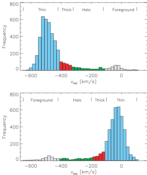
Figure 5. Histograms for both heliocentric (top panel) and disc lag (bottom panel) velocities of all stars within our sample of 21 fields. Regions expected to be inhabited by thin-disc (light blue), thick-disc (red), halo (green) and MW foreground (grey) are highlighted.
