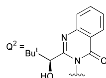
Scheme 1 Atkinson's aziridination.
