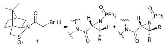
Scheme 1 Atkinson's aziridination.
