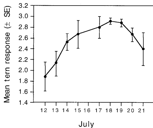
FIGURE 2. Mean daily tern response scores to gulls during the chick stage. No data were collected on 16 July.
