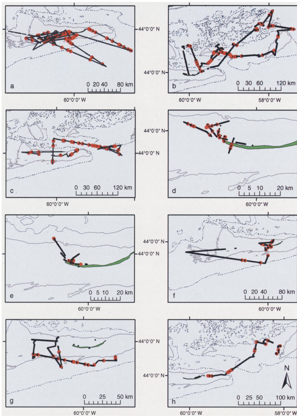
FIG. 2. Movement paths of gray seals, with feeding locations indicated by solid red circles; 100-m (dashed line) and 50-m (gray line) isobaths are also shown. (a) Seal 5114, duration = 30.5 d, n = 87 ; (b) seal 6124, duration = 31.4 d, n = 69 ; (c) seal 24, duration = 30 d, n = 42 ; (d) seal 5687, duration = 32.5, n = 30 ; (e) seal 6122, duration = 32, n = 14 ; (f) 5110, duration = 14 d, n = 21 ; (g) seal 5684, duration = 17, n = 30 ; (h) seal 6125, duration = 8.5, n = 36 . Values of n are the numbers of observations for each seal.
