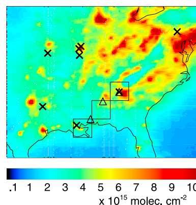
Figure 2. Mean tropospheric NO 2 column over the United States from the OMI SP averaged over the period 2005–2006. Symbols show the location of rural SEARCH (triangles) and EPA/AQS (crosses) sites. The boxes show the GEOS-Chem 2^\circ \times 2.5^\circ horizontal grid representing the SEARCH domain.
