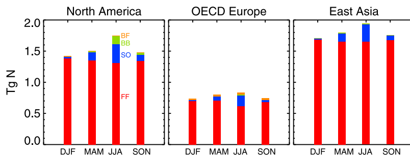
Figure 6. Seasonal NO x emissions for 2005–2006 from surface sources over land of North America, OECD Europe, and East Asia for various source categories: fossil fuel combustion (FF), soil (SO), biomass burning (BB), and biofuel (BF).
